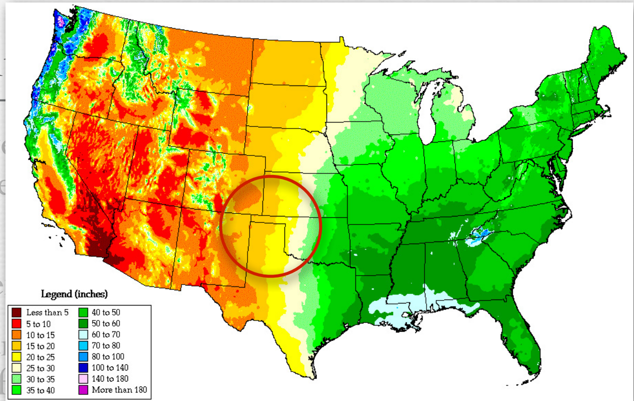
average annual rainfall, 1961-1990
