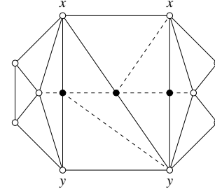
Figure 7: A triangulation of the 2-sphere after removing a vertex of degree k = 8 . There are three edges xy that are cut into two each to restore three-connectedness.
