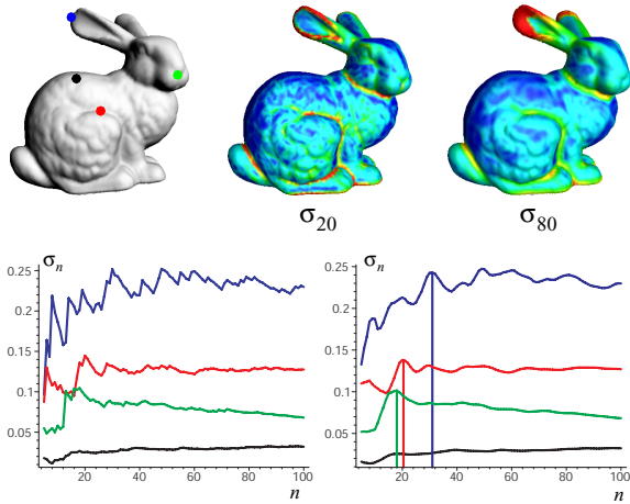
Figure 7: Multi-scale surface variation. The left diagram shows values of \sigma_n for different points on the bunny as a function of neighborhood size n . To avoid instabilities in the detection of local maxima, these curves have been pre-smoothed as shown on the right. The vertical lines show the scale of the extracted maxima in surface variation.
