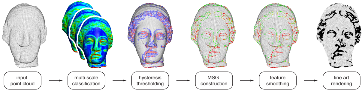
Figure 1: Feature extraction pipeline.
