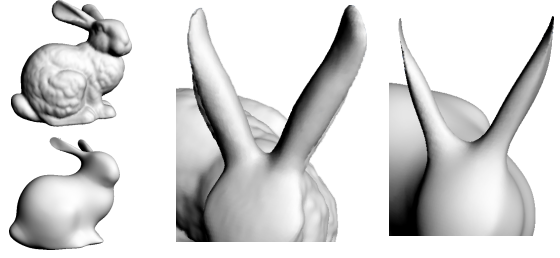
Figure 3: Volume shrinkage leads to increased curvature at the bunny’s ears for iterative Laplacian smoothing.
