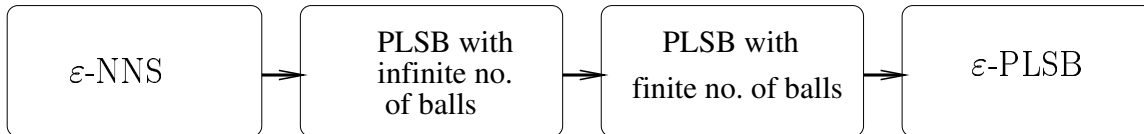
Figure 3: The reduction of \varepsilon -NNS to \varepsilon -PLSB – the intermediate steps illustrate the proof strategy.
