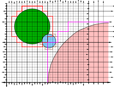
Figure 6: \varepsilon -PLSB data structure
