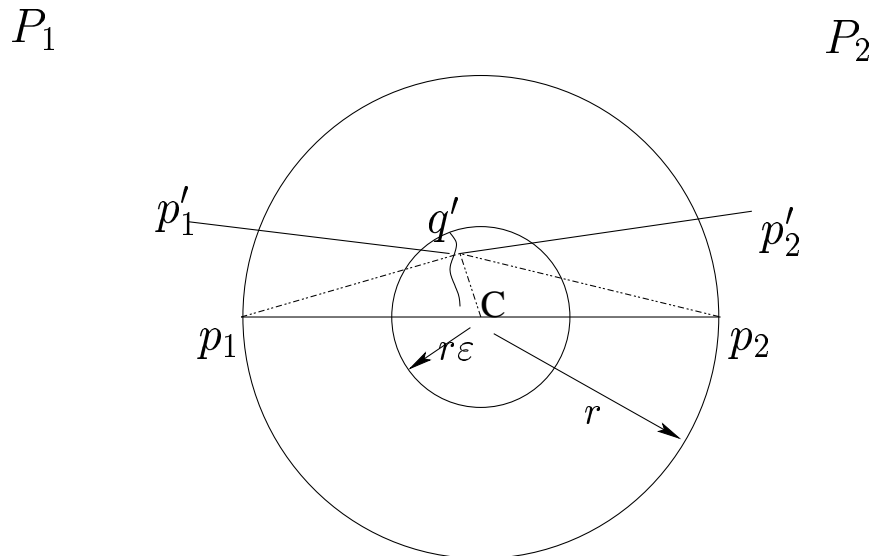
Figure 5: A cut in an approximate MST
