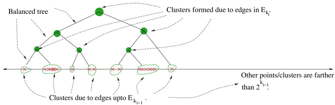
Figure 4: Linear Hierarchical clustering for points in a line
