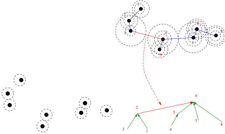
Figure 1: Constructing the cluster tree
