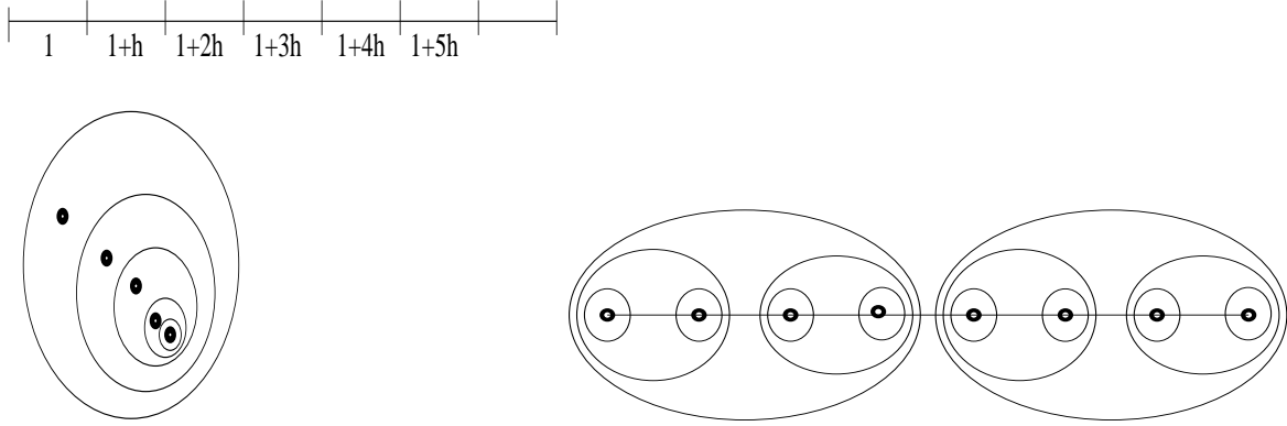
Figure 2: Two different clustering for almost equidistant points in a line
