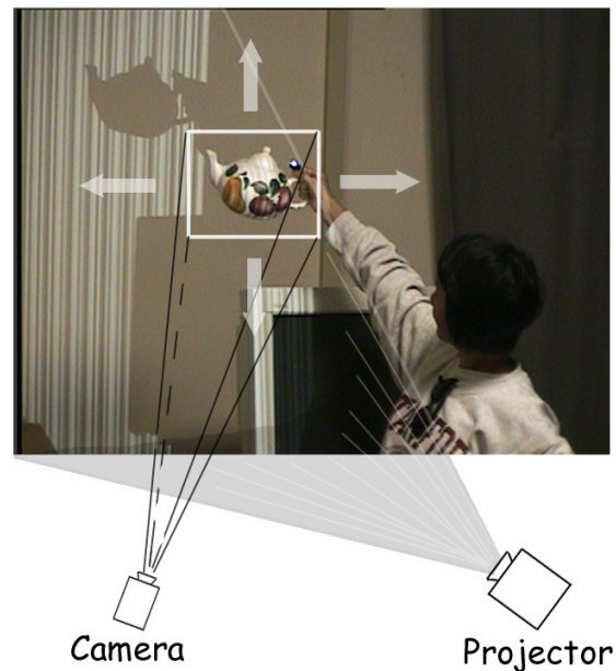
Figure 5 In this foveated structured light depth imager, the projected light covers the entire working volume. The detailed observation system observes only a small region of the entire volume, providing higher resolution depth estimates.
