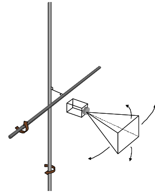
Figure 4. The camera's pan-tilt mechanism is modeled as a pair of arbitrary axes in space. Changes in the camera's pan-tilt parameters cause the camera's position and orientation to rotate around these axes.
