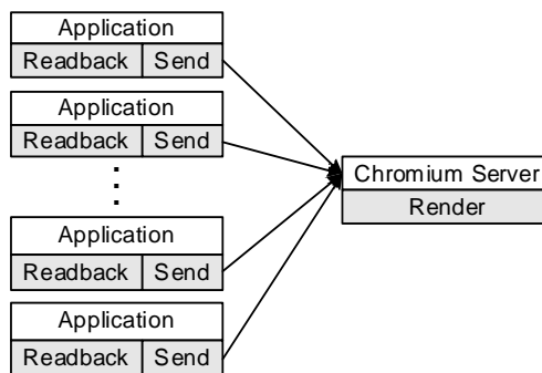
Figure 3: Another possible Chromium configuration. In this example, nodes in a parallel application render their portion of the scene directly to their local hardware. The color and depth buffers are then read back and transmitted to a final compositing server, where they are combined to produce the final image.
