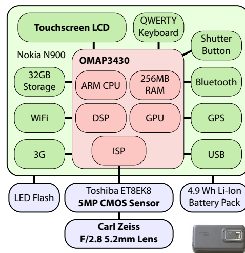
Figure 4: The Nokia N900. The Nokia N900 incorporates similar electronics to the F2, in a much smaller form factor. It uses the same OMAP3430 SoC, an 800 \times 480 touchscreen LCD, and numerous wireless connectivity options. The key strengths of the N900 are its small size and wide availability.
