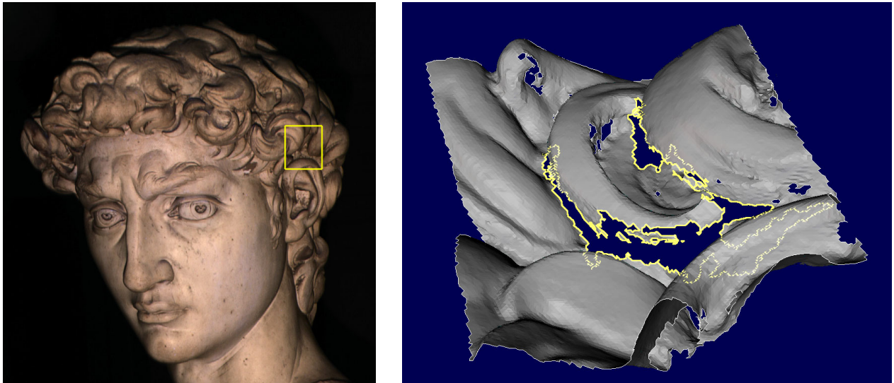
Figure 1: At left is a photograph of the head of Michelangelo’s David. At right is a rendered 3D model of a section of his hair (corresponding to the square in the photograph). The section is 75mm wide on the statue, and the spacing between triangle vertices is 1.0mm. Although this surface was scanned dozens of times (from many different angles), occlusions prevented access to the deepest crevices. The hole highlighted in this rendering has a complex shape and multiple boundary components, i.e. islands floating in the hole. The largest boundary component contains 905 edges. (Hidden portions of this boundary are indicated with broken lines.)
