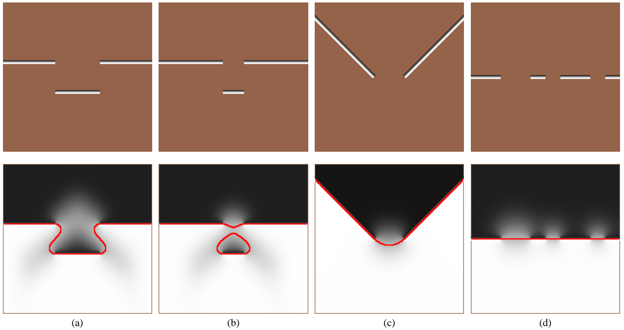
Figure 6: Examples of diffusion in 2D for several kinds of holes. Above: source term; below: diffusion result with zero set marked in red. (a) A frontal (i.e. perpendicular) scan of a surface with a recessed portion leads to two holes, which our diffusion algorithm fills with curved steps. (b) If the recessed portion is sufficiently narrow, the diffusion algorithm instead builds a bridge across it. (c) If two angled surfaces are scanned frontally (relative to each surface), the joint between them may be missed. Our algorithm fills this hole with a smooth fillet. (d) A flat surface with several holes, which is filled with the expected geometry.
