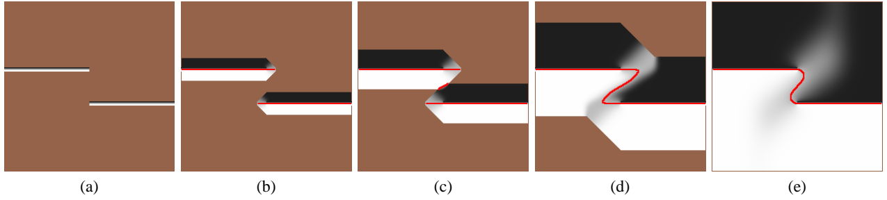
Figure 4: Illustration of 2D diffusion in progress. (a) The source term. Grayscale values encode signed distance, with black and white corresponding to outside ( d = -1 ) and inside ( d = 1 ), respectively. Brown denotes invalid voxels ( v = 0 ). (b) Our diffusion process extends the two surfaces. The red curve marks the zero set. (c) The surfaces begin to interact. (d) The hole closes. (e) The shape is converged.
