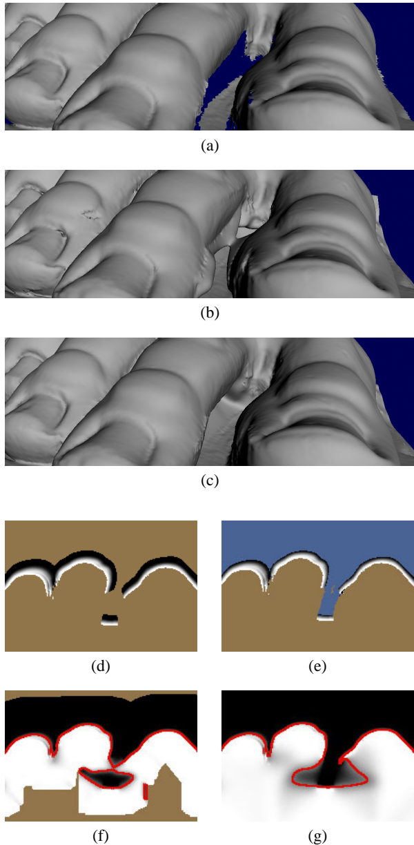
Figure 9: Using line-of-sight constraints. (a) Between two of David’s toes, occlusion causes a hole with ambiguous topology. (b) Filling the hole results in an inappropriate bridge. (c) The addition of line-of-sight information forces the correct topology. (d,e) Slices of the source volume without and with this constraint, respectively. (f,g) The same slices of the diffused volume. Note the bridge that forms in (f) but is avoided in (g). Further diffusion will reduce the protrusion in (g) near where the bridge formed in (f).
